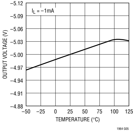
LT1964-5 Output Voltage
